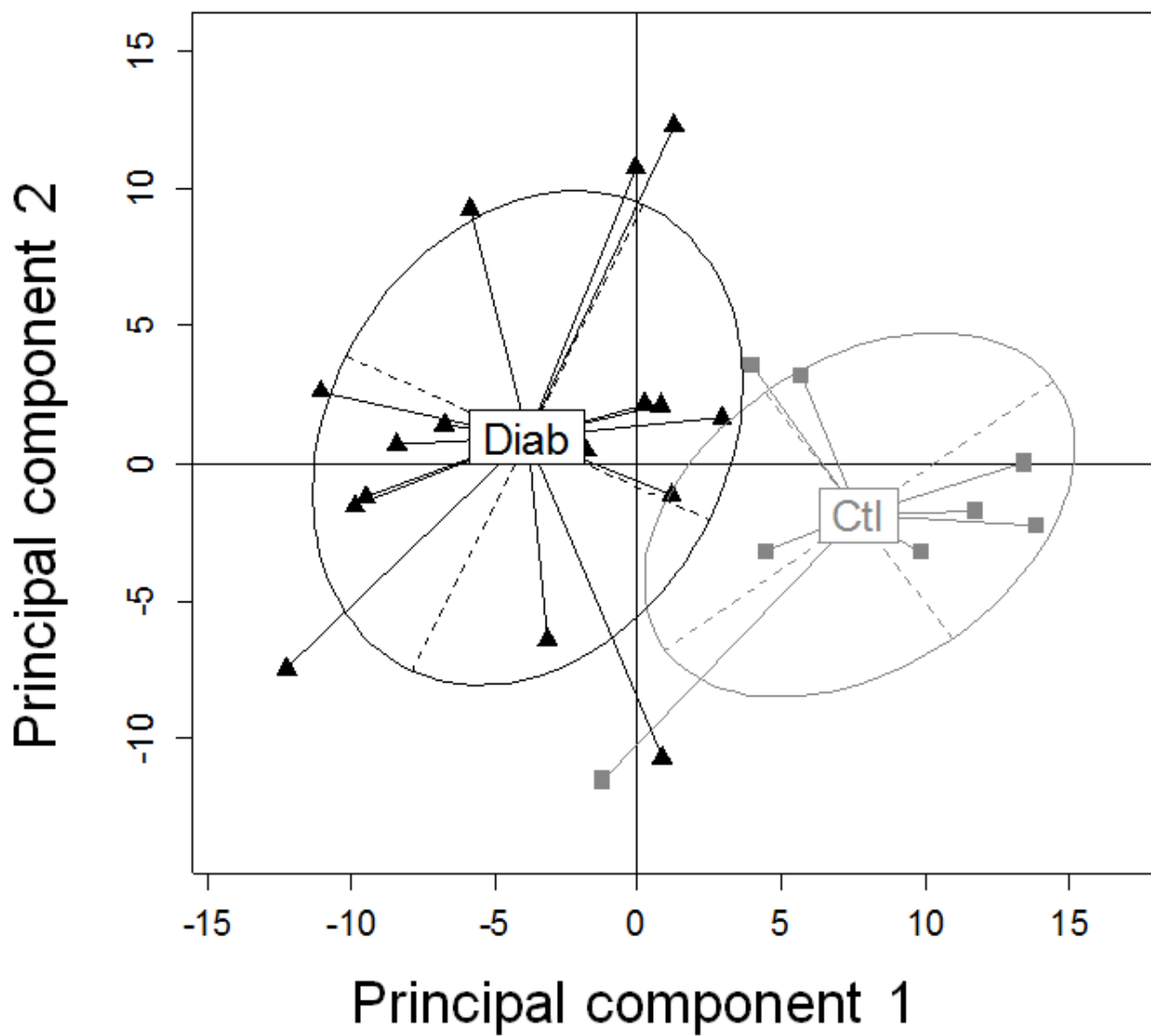
Supplementary Figure 1. Plot of the PCA components.
